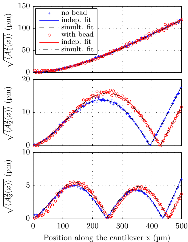
FIG. 7: Amplitude of thermal noise for the first 3 flexural modes along the cantilever A with and without a sphere (in red and blue respectively). The markers represent the data while the lines exhibit the fits : independent fits of each mode in plain line, and simultaneous fit of all modes in dashed line. The agreement is excellent for the bare and the loaded cantilever.
