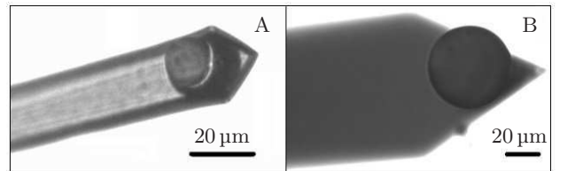
FIG. 5: Pictures from an optical microscope of beads glued at the apex of cantilevers A and B.
