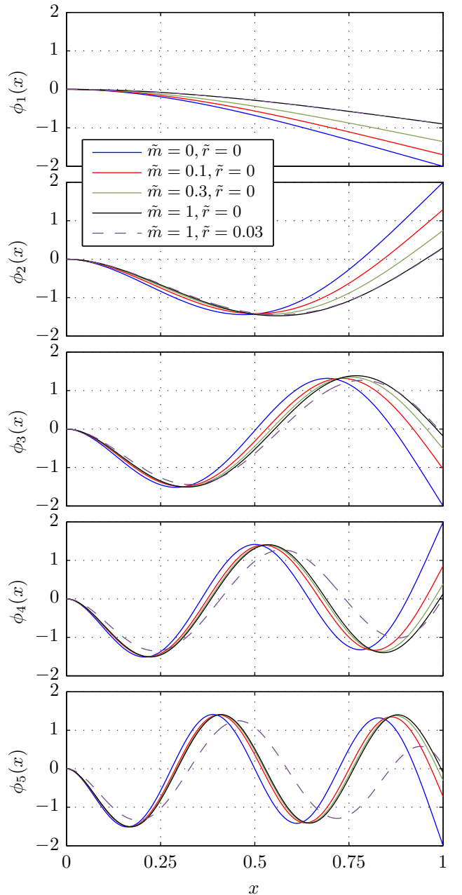
FIG. 2: We plot in this figure the 5 first normal modes \phi_n(x) for various \tilde{m} and \tilde{r} . The amplitude of the first mode decreases and the nodes of the higher order modes get closer to the free end when \tilde{m} or \tilde{r} increase.
