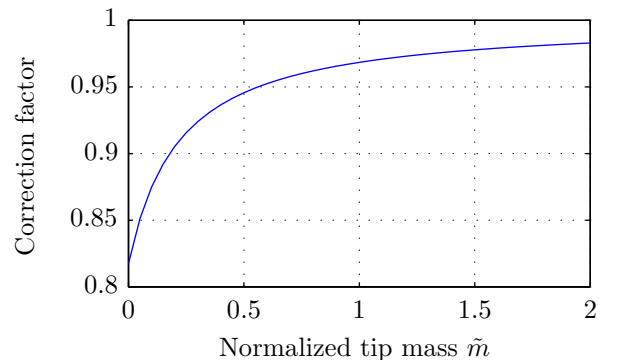
FIG. 9: Multiplicative correction factor to apply to the thermal noise measurement of the first resonant mode with an angular deflection measurement technique to compute the cantilever stiffness: the higher the added mass, the smaller the correction.
