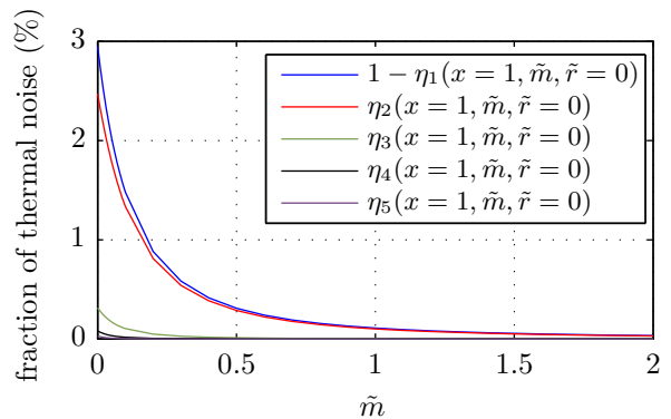
FIG. 4: Fraction \eta_n(x = 1, \tilde{m}, \tilde{r} = 0) at the free end of the cantilever of the mean quadratic deflection driven by thermal noise for the first 5 modes as a function of the normalized bead mass \tilde{m} . The amplitude of the first mode (plotted as 1 - \eta_1 ) quickly overcomes the contribution of all the other modes, for which the inertia of the mass implies a node close to the free end of the cantilever.
