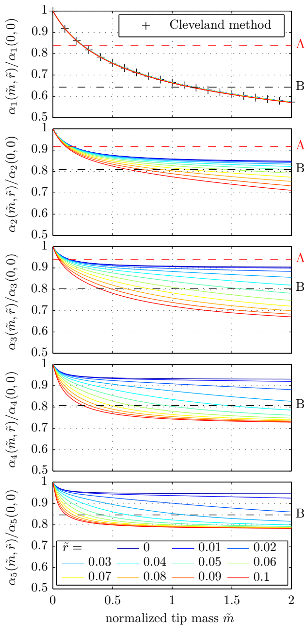
FIG. 10: Spatial eigenvalues \alpha_n(\tilde{m}, \tilde{r}) numerically computed for modes 1 to 5 as a function of \tilde{m} and \tilde{r} , normalized to their value at \tilde{m} = 0 . The values of these ratios for cantilevers A and B, estimated by the frequency shift due to the addition of the bead and supposing an effective length decrease of 2%, are plotted as a labelled horizontal line. Mode 1 is almost independent in the value of \tilde{r} , and can thus be used to estimate \tilde{m} . This curve is very close to the prediction given in the Cleveland method [24].
