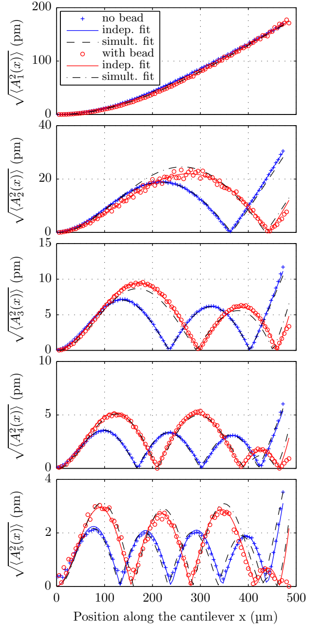
FIG. 8: Amplitude of thermal noise for the first 5 flexural modes along the cantilever B with and without a sphere (in red and blue respectively). The markers represent the data while the lines exhibit the fits : independent fits of each mode in plain line, and simultaneous fit of all modes in dashed line. The agreement is very good for the bare and the loaded cantilever.
