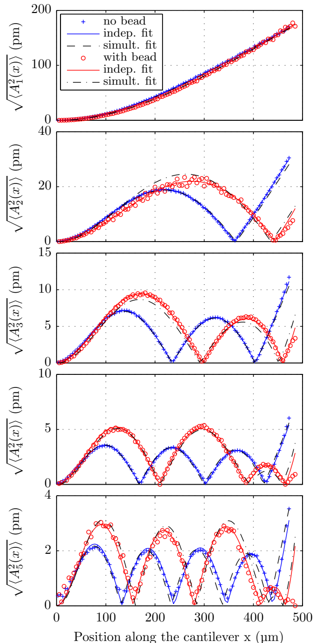
FIG. 8: Amplitude of thermal noise for the first 5 flexural modes along the cantilever B with and without a sphere (in red and blue respectively). The markers represent the data while the lines exhibit the fits : independent fits of each mode in plain line, and simultaneous fit of all modes in dashed line. The agreement is very good for the bare and the loaded cantilever.
