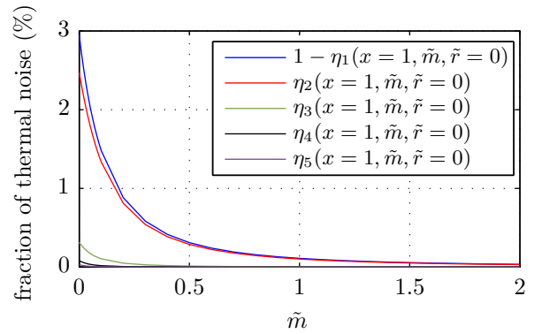
FIG. 4: Fraction \eta_n(x = 1, \tilde{m}, \tilde{r} = 0) at the free end of the cantilever of the mean quadratic deflection driven by thermal noise for the first 5 modes as a function of the normalized bead mass \tilde{m} . The amplitude of the first mode (plotted as 1 - \eta_1 ) quickly overcomes the contribution of all the other modes, for which the inertia of the mass implies a node close to the free end of the cantilever.
