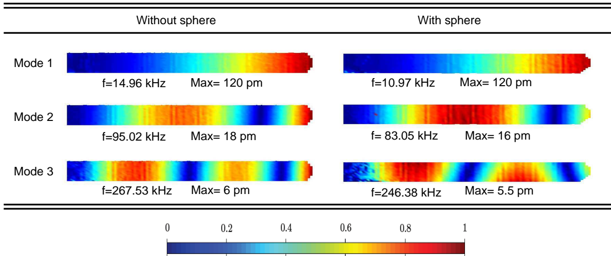
FIG. 6: Maps of thermal noise of cantilever A. The rms amplitude of the first 3 flexural modes, with (right) and without (left) a bead glued at the free cantilever end, are plotted using a color coded amplitude map (color bar at the bottom of the figure). The resonant frequency and full scale amplitude are given below each map. A weak component in torsion can be clearly seen for the third mode with the bead, hinting at a slightly off axis gluing of the colloidal particle.
