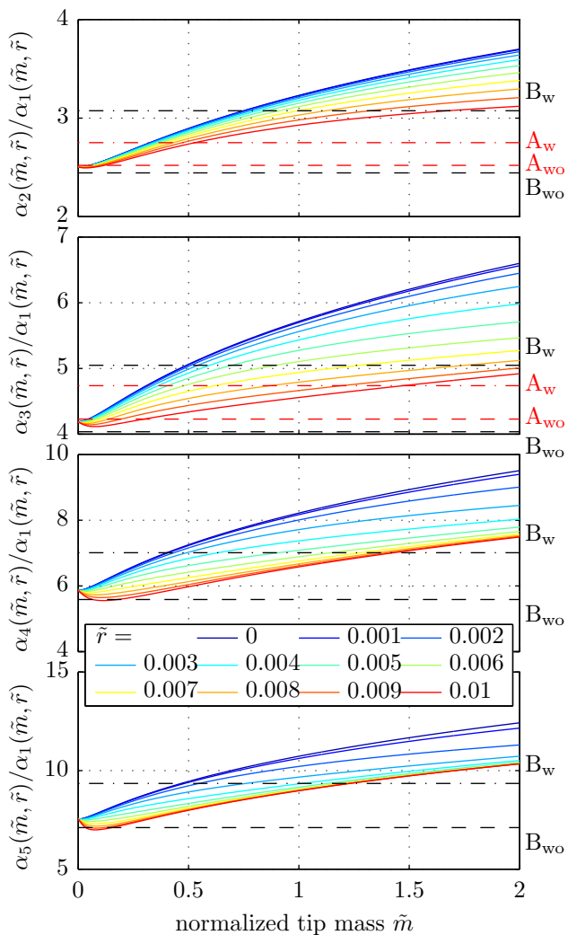
FIG. 11: Spatial eigenvalues \alpha_n(\tilde{m}, \tilde{r}) numerically computed for modes 1 to 5 as a function of \tilde{m} and \tilde{r} , normalized to the value of mode 1. The values of these ratios for cantilevers A and B, estimated by the frequency ratios between modes, are plotted as a labelled horizontal line for unloaded (index _{wo} ) and loaded (index _w ) cantilevers. The model is not suited to the description of bare cantilever B ( B_{wo} ), but allows the estimation of \tilde{m} and \tilde{r} for the 3 other situations.
