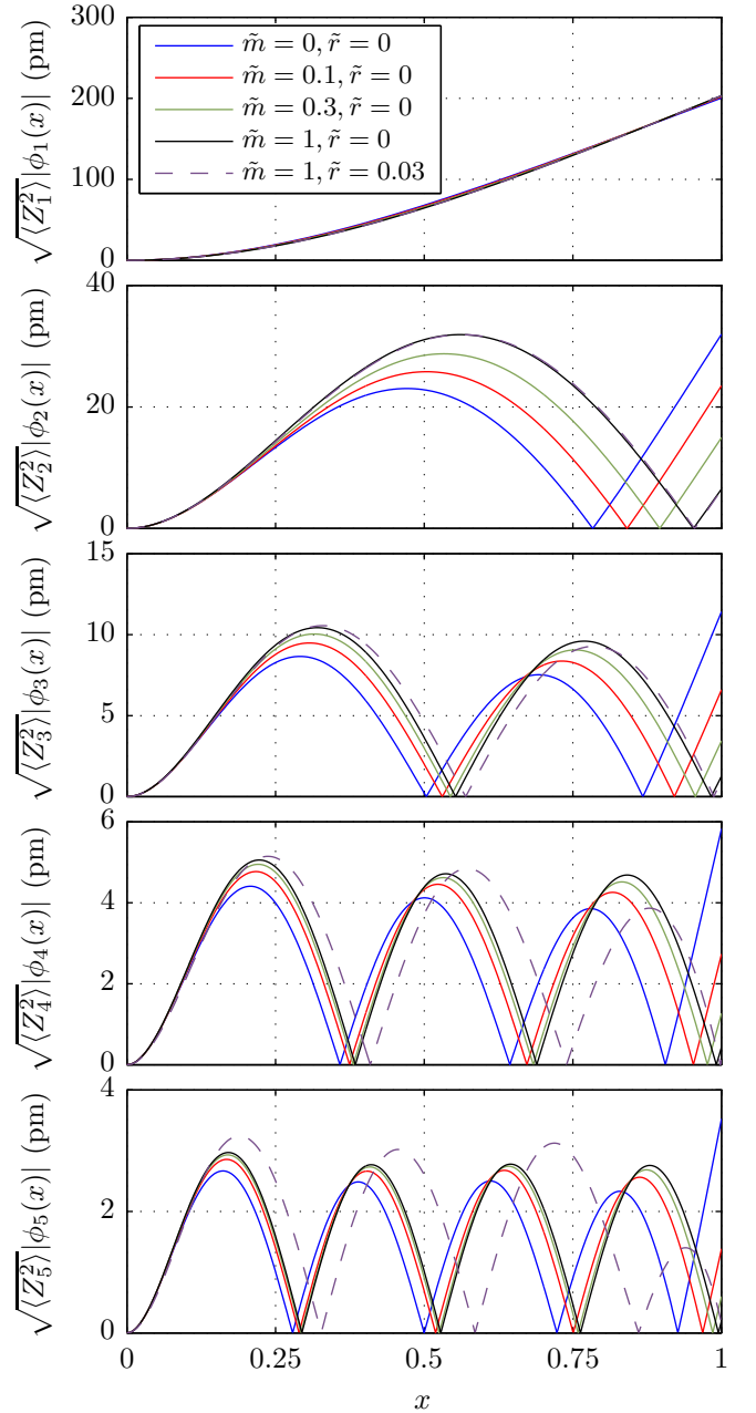
FIG. 3: Thermal noise expected for a cantilever of static stiffness k = 0.1 N/m at 300 K for a few values of \tilde{m} and \tilde{r} . The rms deflection of the first 5 modes is plotted as a function of the position along the cantilever x . The first mode is weakly impacted by the bead. When \tilde{m} increases, the amplitude of the higher order modes vanish at the end, and the thermal energy is reported towards the antinodes, the amplitude of which raises.
