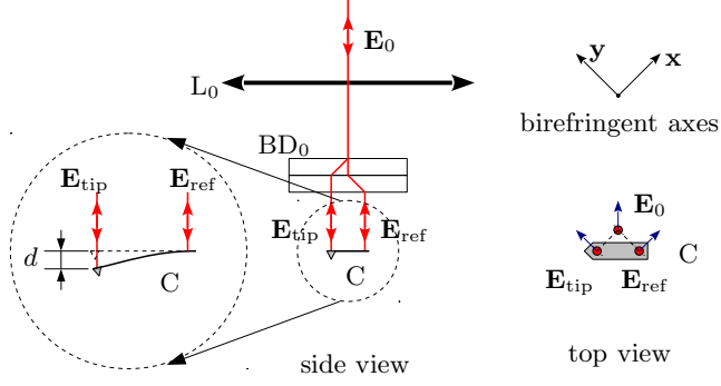
FIG. 1. Measurement area: the incident beam (electric field \mathbf{E}_0 ) is focused on the cantilever C by the lens L_0 . When passing through 2 calcite beam displacers \text{BD}_0 with orthogonal optical axes \mathbf{x} and \mathbf{y} , light is split into 2 parallel beams, which are reflected by the base and free end of the sensor (fields \mathbf{E}_{\text{ref}} and \mathbf{E}_{\text{tip}} ). A deflection d of the cantilever modifies the optical path of the second beam by \delta L = 2d . On the top view, blue arrows show the direction of polarization of each beam, whereas on the side view, red arrows indicate the direction of propagation of light (to and back from the cantilever).
