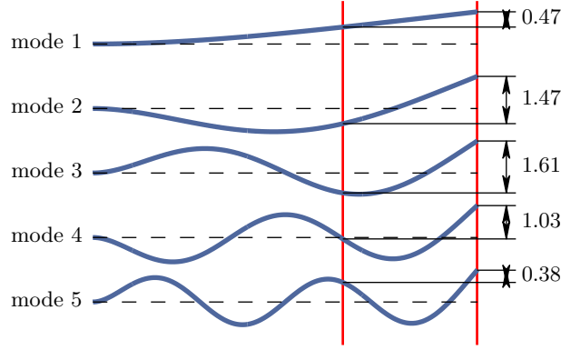
FIG. 10. In the bi-calcite configuration, the distance between the two laser spots is smaller than the length of the cantilever, thus the measured deflection does not correspond to the actual value. The correction to consider is mode dependent: according to the position of the spots with respect to the nodes and antinodes of the spatial shape, it can be smaller or larger than one. Using an Euler Bernoulli model for the mechanical beam, we estimate the coefficient noted on the figure for the measured amplitude normalized to the deflection of the free end for the 5 first modes.
