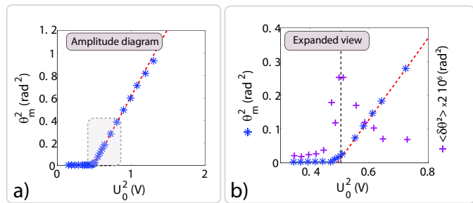
Fig. 2: a) Amplitude diagram of \theta_m^2 versus U_0^2 . Experimental data( \star ) and solution of LG equation with U_c = 0.704\text{V} (red dashed line) b) Expanded view of the plot in (a). The variance \langle \delta\theta^2 \rangle of \theta_m is plotted in b) as a function of U_0^2 . As the amplitude of the fluctuations of \theta_m is very small the plotted values (+) correspond to \langle \delta\theta^2 \rangle \times 2 \cdot 10^6 .
