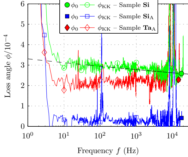
FIG. 7. Internal damping \phi as a function of frequency for the three measured samples. The result of the reconstruction process through Kramers-Kronig's relations \phi_{\text{KK}} is in very good agreement with the Saulson model ( \phi_0 measured with the fitting procedure of the thermal noise at resonance through equation (4)). The dissipation is much weaker after annealing for the silica coating, reaching the limits of our detection system. Peaks around 10 kHz and high noise level below 5 Hz are due to the residual environmental noise.
