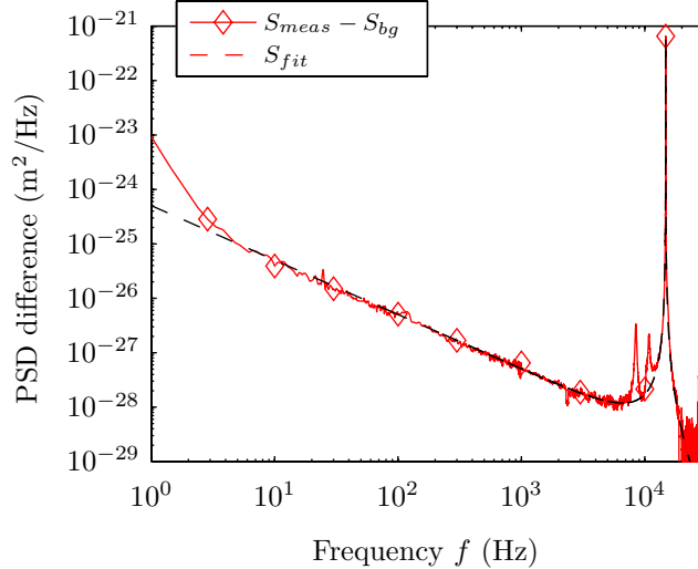
FIG. 6. PSD of sample \mathbf{Ta}_A coated with tantala obtained by subtraction of the averaged PSD of measured signals S_{meas} and averaged PSD of background noise S_{bg} . The fit of the resonance with equation (4) is still valid at low frequencies, demonstrating the frequency independence of \phi . Peaks around 10 kHz and high noise level below 5 Hz are residual environmental noise.
