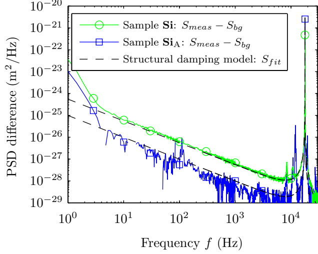
FIG. 5. PSD of samples Si and Si A coated with silica obtained by subtraction of the averaged PSD of measured signals S_{meas} and averaged PSD of background noise S_{bg} (PSDs of figure 4 for sample Si ). The fit of the resonance with equation (4) is still valid at low frequencies, demonstrating the very weak frequency dependence of \phi . The thermal noise of the annealed sample is an order of magnitude lower than that of the as-coated sample, almost reaching the limit of our detection system. Peaks around 10 kHz and high noise level below 5 Hz are residual environmental noise.
