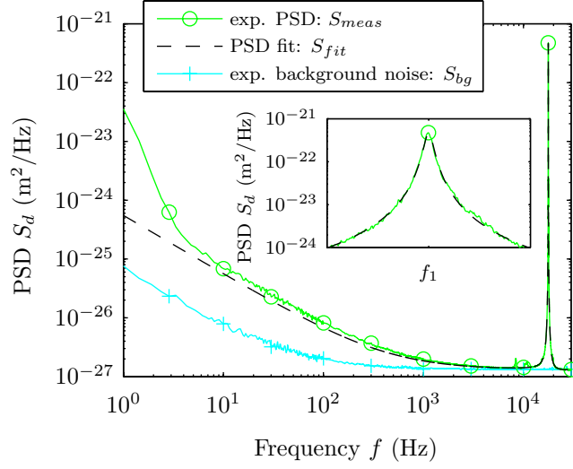
FIG. 4. Averaged PSD of measured deflection for 140 data sets for a silica coated cantilever measured in vacuum (sample Si ). The curve is compared to the fitting function (4) and to the background noise, measured on a rigid mirror. Inset: zoom on a 100 Hz frequency interval around resonance.
