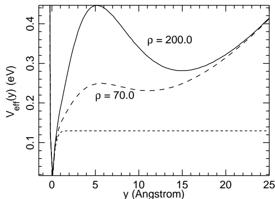
Fig. 17. Effective potential of the PBD model with a Morse intra-pair potential V_M and a nonlinear stacking interaction W for two values of \rho . The dotted line shows the Morse potential V_M for D = 0.13 eV, \alpha = 4.2 \text{\AA}^{-1} . The full line shows the effective potential V_{\text{eff}}(y) (Eq. (8)) for K = 0.00045 eV \text{\AA}^{-2} , \delta = 0.4 \text{\AA}^{-1} and \rho = 200 . The parameters of the model have been chosen to give a denaturation transition temperature T_c \approx 340 K, which is a realistic value for DNA. The dash line shows V_{\text{eff}}(y) for a smaller value \rho = 70 , all other parameters being unchanged.
