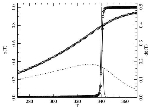
Fig. 2. Melting curves of homopolymer poly-A DNA calculated with the PBD and PB models. Full line with circles: fraction \phi(T) of open base pairs versus temperature calculated with the PBD model using the parameters of table I. A base pair is defined as open when its average stretching is beyond 1.5 \text{ \AA} . The full line without symbols is the derivative versus T of \phi(T) . Dash line with triangles: fraction of open base pairs calculated with the PB model, i.e. by setting \rho = 0 in the parameters. As this also slightly changes the transition temperature, the parameter D_{AT} = 0.105 \text{ eV} has been selected for this calculation instead of D_{AT} = 0.12905 \text{ eV} for the PBD model to get similar transition temperatures for both cases. The dash line without symbols shows the derivative of the melting curve for the PB model, magnified by a factor 20 to make it visible on the same vertical scale as d\phi(T)/dT in the PBD case.
