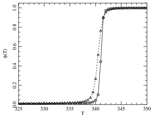
Fig. 5. Comparison of the melting profiles for poly-A DNA sequences computed with the modified PBD model with a closing barrier (full line with circles) and the PBD model with the Morse potential (dotted line with triangles)
