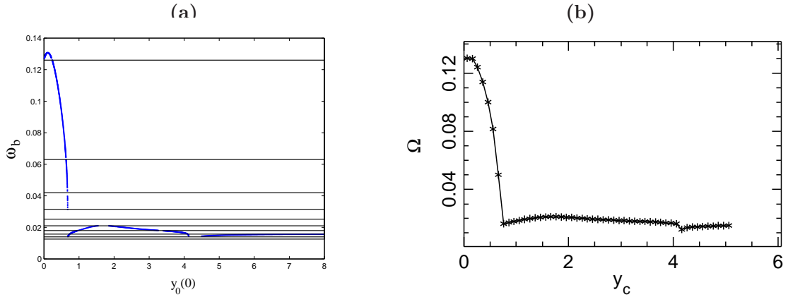
Fig. 16. (a) Frequency \omega_b of breather solutions of equation (10) numerically computed by the Newton's method [29], as a function of breather amplitude y_0(0) (expressed in \text{\AA} ). Resonances with phonons, represented by black bands, prevent the existence of breathers (only the first ten resonance bands have been represented for clarity). Parameters are \alpha = \sigma = 4 \text{ \AA}^{-1} , D = 0.0857 \text{ eV} , E = 4 \text{ eV \AA}^{-1} . Particle masses are set to m = 300 atomic mass units and K = 0.01 \text{ eV \AA}^{-2} . (b) Frequency of the breathers obtained numerically by exciting only the central particle of the lattice, as explained in Sec. 2.4. The numerical results given by the two different methods are in excellent agreement.
