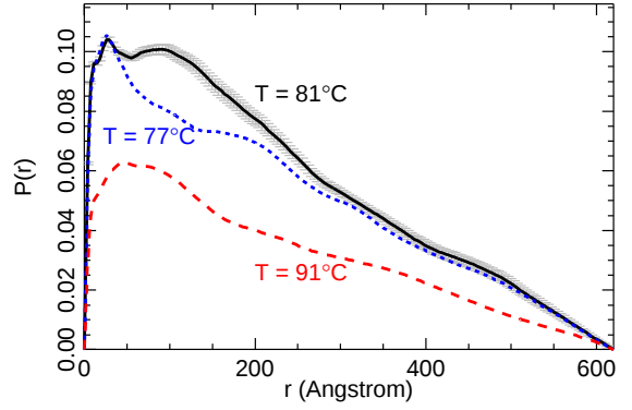
Fig. 4: The pair-distance distribution function P(r) for sequence B at three temperatures: blue dotted line, T = 77^\circ\text{C} , black full line T = 81^\circ\text{C} , red dash line T = 91^\circ\text{C} . The error bars for the case T = 81^\circ\text{C} show the error computed by the GNOM program.
