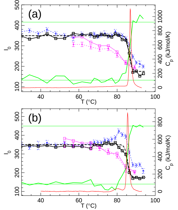
Fig. 3: Results of the calorimetry and analysis of the SAXS data for sequence A (a) and sequence B (b). The red lines show the specific heat measured by calorimetry. The squares and black lines show the variation of I_0(T) on heating, deduced from the fit in q space. The black dashed lines show a fit of those data with the sigmoidal curve I_{\text{fit}}(T) (Eq. 6). The magenta squares and full line show I_0(T) from the measurements made on cooling from the highest temperature. The blue circles and dotted lines show I_0(T) deduced from the analysis in real space for the measurements on heating, and the magenta dots and dashed lines show I_0(T) deduced from the analysis in real space for the measurements on cooling. The green full lines show the variation of the fraction of fully open molecules, on a scale going from 0 to 1 (marked by the two green horizontal lines), obtained from Eq. 4, computed with the results of the analysis in q space.
