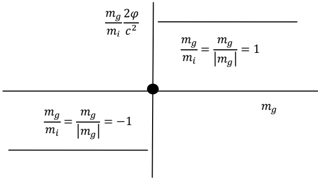
Fig. 2: Anti-symmetry of the ratio \frac{m_g}{m_i} . To simplify the representation on this graph, we took into account the principle of equivalence but a more general representation would be a cloud of possible points distributed anti-symmetrically.
