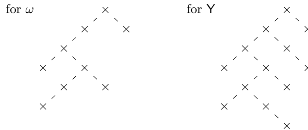
FIGURE 4. The bijection LToBz from lambda terms to zigzag free trees
