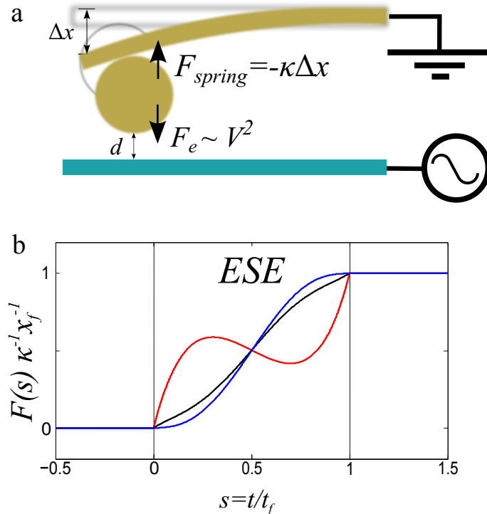
FIG. 1: a- Sketch of the experimental setup. The cantilever-sphere system is connected to ground, while the surface is connected to the signal generator. The external force is applied by the voltage difference between them. b- Force ESE protocol for different final times t_f = 0.2 ms (red), 0.5 ms (black) and 2 ms (blue) as a function of the normalized time s = t/t_f . If we reduce enough the protocol time, the inertial term of the protocol becomes dominant and yields a non monotonous force, see the red curve.
