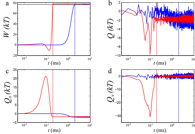
FIG. 4: Energetics of the system along the ESE route. a Average value of the cumulative work as a function of time for different protocol times t_f . Horizontal black line represents the difference of free energy between the initial and final state \Delta\mathcal{F} . b Average value of the cumulative total heat. c Average value of the cumulative potential heat. d Average value of the cumulative kinetic heat. Its importance reduces once we increase the protocol time. The kinetic heat is compensated with the potential one, showing the classical oscillation of a classical harmonic oscillator. In the four graphs, red lines are for t_f=0.2 ms and blue lines for t_f=2 ms.
