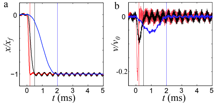
FIG. 3: Comparison of the ESE protocols at various t_f . a- Ensemble average of the trajectory over 5000 realizations for t_f = 0.2 ms (red), t_f = 0.5 ms (black) and t_f = 2 ms (blue). The higher modes starts to dominates the dynamics of the system once the protocol is shorter than 2\pi/\omega_o \simeq 0.4 ms. b- Ensemble average of the normalized velocity for the same times than a). The normalized velocity \dot{x}(t)/v_o allows a better vision of the higher orders effect. In both figures, the vertical lines represent the end of each protocol. All processes start at t = 0 ms.
