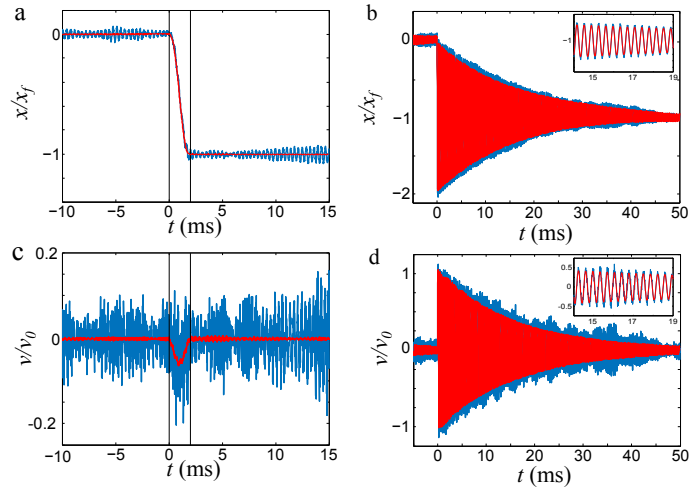
FIG. 2: Dynamics of the system along the STEP and ESE protocols. All processes start at t = 0 ms. a- Position evolution along the ESE process with t_f = 2.0 ms. b- Position evolution along the STEP protocol. Intrinsic oscillations of the cantilever are much faster than the dissipation process what makes difficult to distinguish the trajectory. The inset provides a magnification of a small region. c- Normalized velocity \dot{x}(t)/v_o as a function of time, along the ESE process. d- Normalized velocity velocity evolution along the STEP process. The inset increases the time resolution, to observe the intrinsic oscillations. All figures show the dynamics of a single realization (blue) and the ensemble average over 5000 realizations (red). Vertical black solid lines in a and c represent the limits of the ESE protocol ( t_f = 2 ms).
