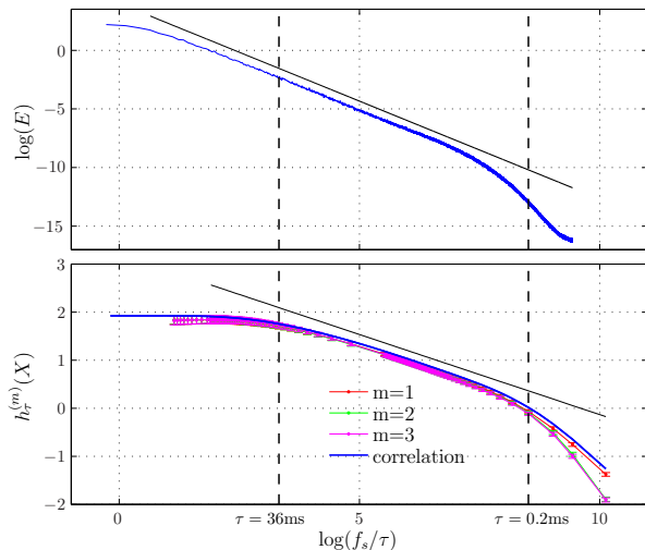
Figure 2: Top: Power Spectral Density of the experimental signal. The straight line corresponds to the K41 scaling. Bottom: entropy rate h_\tau^{(m)} , as a function of the scale ( f = f_s/\tau ) for different embedding dimensions m \in \{1, 2, 3\} . The blue curve corresponds to eq.(3) using the autocorrelation function. The straight line is a line of slope -1/3 .
