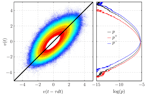
Figure 1: Left: bi-variate PDF of (v(t), v(t - \tau dt)) . Right: p(X) (in red), p_+(X) (blue) and p_-(X) (black).
