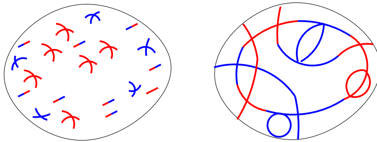
Ising model on random graphs
