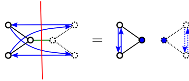
Figure 5: Any unlabelled \mathcal{E} = \text{SET}_{\{2\}}^{\circledast} \circledcirc \mathcal{A}_{\Omega^*} object corresponds to two identical copies of a cycle-pointed Pólya tree.
