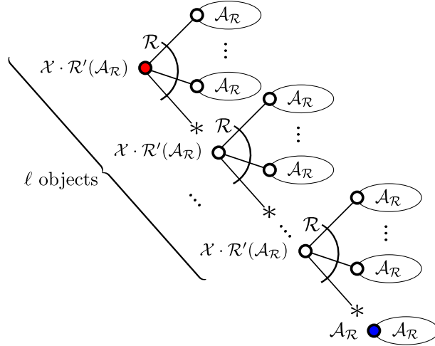
Figure 6. The decomposition of \mathcal{A}_R^{(\ell)} .
