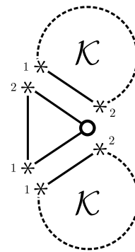
Figure 3. Decomposition of the class \mathcal{K}^\circ for k = 2 .
