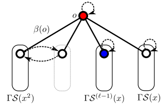
Figure 7. The sampler \Gamma \mathcal{S}^{(\ell)}(x) .
