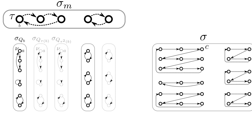
Figure 1. Composition of cycles.
