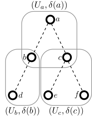
Figure 8. Patching together discrete metric spaces.
