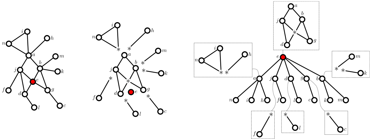
Figure 2. Correspondence of rooted connected graphs and enriched trees.
