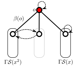
Figure 5. The sampler \Gamma \mathcal{S}(x) .
