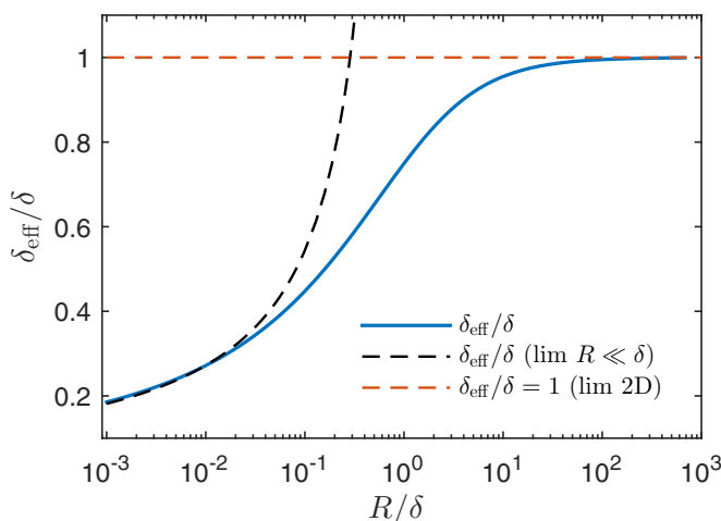
FIG. 8. Plot of \delta_{\text{eff}}/\delta as given by Eq. (11) as a function of R/\delta (solid blue curve). The dashed red line displays the 2D regime for which \delta_{\text{eff}} = \delta and the dashed black curve displays the small radius asymptotic regime as given by Eq. (12).
