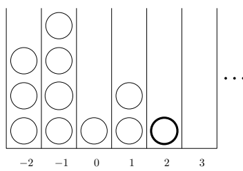
(c) The configuration \Phi_2(X) .
