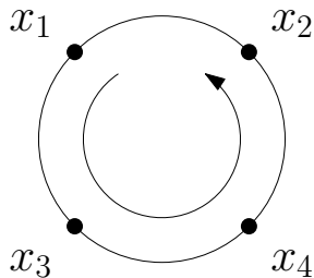
Figure 1: A cyclic order Z on X_n may be represented pictorially by placing all the x_i 's on a circle, in such a way that (x_i, x_j, x_k) \in Z if and only if starting at x_i and turning in the positive direction, one sees x_j before x_k . Here n = 4 and Z is the set formed by the union of the four triples (x_1, x_3, x_4) , (x_3, x_4, x_2) , (x_4, x_2, x_1) and (x_2, x_1, x_4) with the eight possible cyclic permutations of these four triples. The arrow indicates the positive direction of rotation. The cyclic order Z belongs to the following sets : \mathcal{P}_{-+} , \mathcal{Q}_{-+}^+ and \mathcal{R}_{-+}^{+-} .
