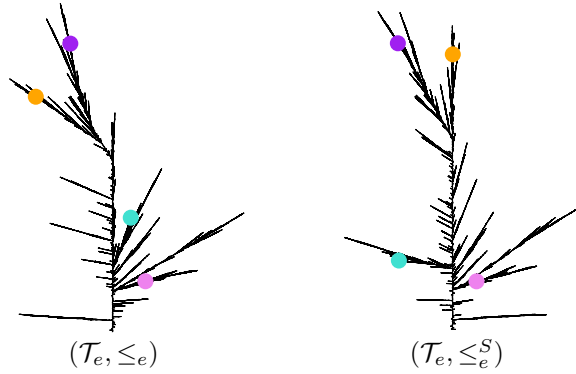
FIGURE 5. The tree \mathcal{T}_e , drawn according to the two orders \leq_e and \leq_e^S . Four points have been marked. The data is the same as in fig. 4.
