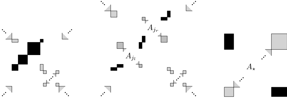
FIGURE 7. Left: B_i for i \in I , in the case s_i = \oplus , i = j_l for some j . Center: B_j for j \in J , in the case s_j = \oplus , j = j'_l for some j' . Right: B_0 , in the case s_* = \oplus .
