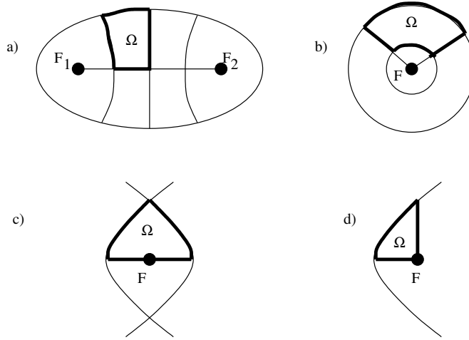
Figure 1: Examples of confocal planar billiards; F_1 , F_2 , F are the foci; the conics in c) and d) are parabolas. All of these billiards have quadratic integrals, except for the billiard at Fig. 1d), which has a degree 4 integral.
