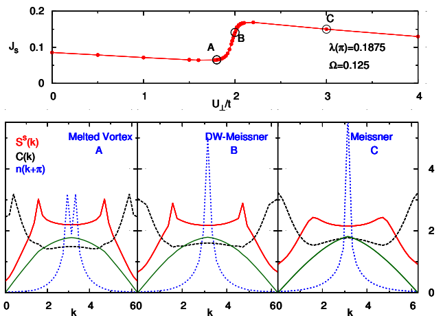
FIG. 6. Upper panel shows the spin current J_s as a function of strength of interchain interaction, solid red line is only a guide to eye. Panels below show 8S^s(k) (red solid line), 4C(k) (black dashed line), and n(k) (blue dotted line) where the argument of this last quantity has been shifted of \pi . Left, center and right panel shows these quantities for the cases indicated by the point A, B and C in the upper panel, respectively corresponding to cases where the system is in the melted Vortex phase, in the CDW-Meissner phase and in the Meissner phase. Data shown are from DMRG simulations in PBC for L=32 . Color online.
