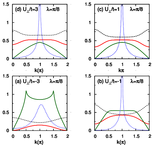
FIG. 5. S^c(k) and S^s(k) are respectively shown as dark-green and red solid lines in all panels. Blue dotted lines are for spin resolved momentum distribution n_\sigma(k) whose argument has been shifted shifted of \pi and black dashed lines are for rung-rung correlation function C(k) . Panels a , b , c and d are respectively for U_\perp = -3, -1, 1 and 3 . Data from L = 64 DMRG simulations in PBC at \lambda = \pi/8 , for \Omega/t = 0.5 and \rho = 0.5 . Color online.
