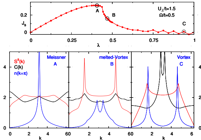
FIG. 7. Upper panel shows the spin current J_s as a function of the applied flux, red line is only a guide to eye. Panels below show S^s(k) (red solid line), C(k) (black line), n_{\sigma}(k) (blue line) where the argument of this last quantity has been shifted of \pi . Left, center and right panels show these quantities for the cases indicated by the point A , B and C in the upper panel, respectively corresponding to cases where the system is in the Meissner phase, in the melted-Vortex phase and in the Vortex phase. Data shown are from DMRG simulations in PBC for L=64 . Color online.
