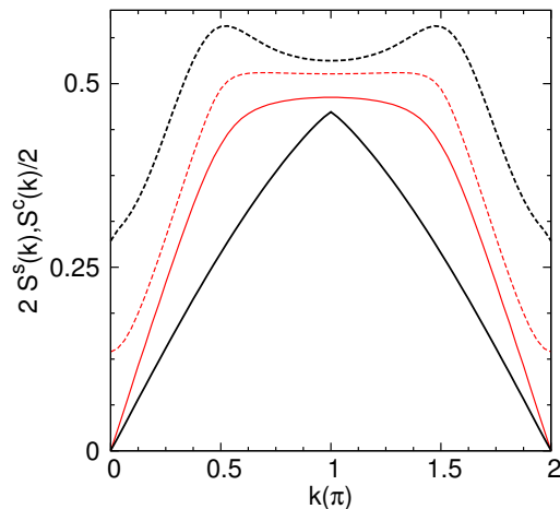
FIG. 4. S^c(k) and S^s(k) for the repulsive case, respectively solid and dotted lines, for U_{\perp}/t = 0.5 and 5.5 , red and black curves respectively. Data from L = 64 DMRG simulations in PBC at \lambda = 0.0625\pi , for \Omega/t = 0.125 and \rho = 0.5 . Color online.
