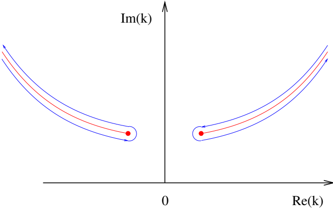
FIG. 8. The integration path in complex k plane for h > m . The red curves are such that E_-(k)^2 < 0 . The red dots at extremities of the curve are the points where E_-(k) = 0 .
