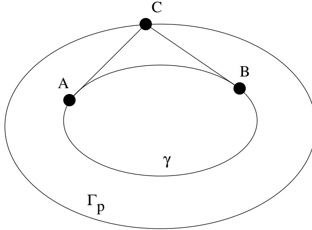
Figure 1: The string construction.
