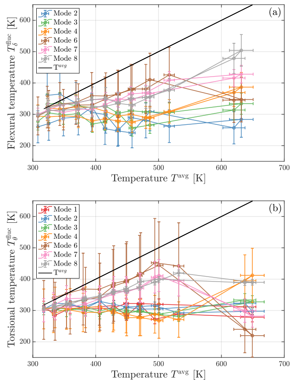
FIG. 4. Fluctuation temperature vs. average temperature. In figure (a), the flexural T_n^{\text{fluc}} is shown with respect to T^{\text{avg}} . The black line represents the “equilibrium” temperature, i.e. the fluctuations an object would show had it been in thermal equilibrium with a thermal bath at T^{\text{avg}} . All the modes lie below this line, as if there was a dearth of thermal noise. The modes shown span from 2 to 8, excluding mode 5 because of the laser probe being on a node of sensitivity. In figure (b), the same scenario is shown for the torsional degrees of freedom (and mode 5 is omitted for the same reason). The apparent crossover between mode 4 and 6 at the highest T^{\text{avg}} is interpreted as a small drift in the laser position, see Appendix B for details in computing T^{\text{fluc}} and uncertainties.
