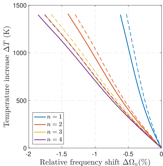
FIG. 6. Functions g_1^{-1} to g_4^{-1} computed for a silicon cantilever heated at its extremity ( x_0 = L ) in vacuum, supposing l_{th} = L/20 (plain line) or l_{th} = 0 (dashed lines). Because of the non-uniform temperature along the cantilever, the relative frequency shift is mode dependent. These functions are independent of the geometry and can be used for any silicon cantilever to infer \Delta T (and thus the full temperature profile) from a measurement of \Delta\Omega_n .
