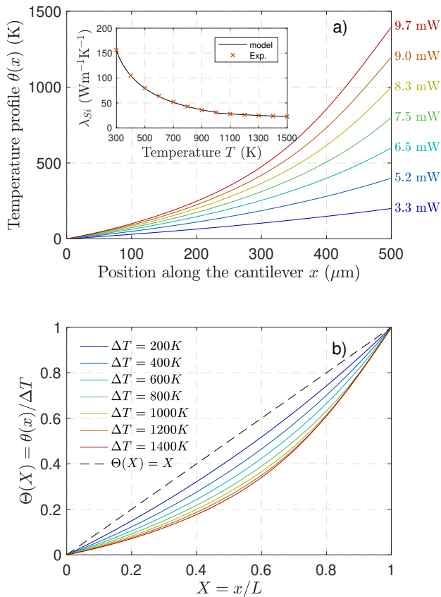
FIG. 1. a) Numerical temperature profiles computed for a silicon cantilever in vacuum with L = 500\mu\text{m} and BH = 75\mu\text{m}^2 , heated at x_0 = L by a constant power P_a labelled on the right of each curve. The only thermal transfer process taken into account here is conduction, and we assumed T(x = 0) = T_0 = 22^\circ\text{C} . Inset: temperature dependence of the silicon conductivity \lambda from Refs. 44 and 45. b) Temperature profiles of panel a) normalized by their respective maximum temperature increase \Delta T = \theta(x = L) . They clearly deviate from the linear profile \Theta(X) = X (dash curve) which would correspond to a material with constant thermal conductivity.
