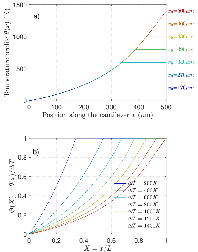
FIG. 2. a) Numerical temperature profiles computed for a silicon cantilever in vacuum with L = 500\mu\text{m} and BH = 75\mu\text{m}^2 , heated by a constant power P_a = 9.7\text{mW} at position x_0 labelled on the right of each curve. The only thermal transfer process taken into account here is conduction, and we assumed T(x = 0) = T_0 = 22^\circ\text{C} . b) Temperatures profiles of panel a) normalized by their respective maximum temperature increase \Delta T = \theta(x = L) .
