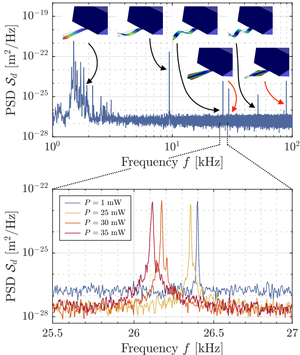
FIG. 2. Experimental thermal noise spectra. (a) The Power Spectral Density (PSD) of d displays various resonance peaks, which we can distinguish between the flexural ones (black arrows) and torsional ones (red arrows). The first resonance n = 1 is plagued by low-frequency noise and is thus discarded in the analysis. (b) Increasing the laser power causes a redshift in the resonance frequencies of the modes (in this case n = 3 ) as the Young's modulus of silicon decreases with temperature.
