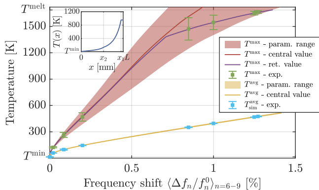
FIG. 5. Estimation of T^{\text{avg}} and T^{\text{max}} : from the parametric sweep reported in Table I, we estimate the possible values of the average (yellow curve) and maximum temperature (red curve) of the cantilever, and at the same time the frequency shift for the mode numbers 6 to 9. The dispersion of T^{\text{avg}} (yellow shaded area) is small. As a result, the error associated to the experimental value of T^{\text{avg}} at a given frequency shift (cyan squares) is also small. Conversely, the estimation of T^{\text{max}} yields a wide parameter range (red shaded area). No bijective relation is possible, thus we estimate T^{\text{max}} as the average of a uniformly distributed variable between the possible values at a given frequency shift. The purple curve represents the retained value of T^{\text{max}} for each frequency shift and the green squares are the experimental values. In the inset we show a typical temperature profile T(x) , with each of the two laser beams (at x_1 and x_2 ) injecting an absorbed power of 15 mW. We can see how T(x) is highly non-linear and peaked at the heating points.
