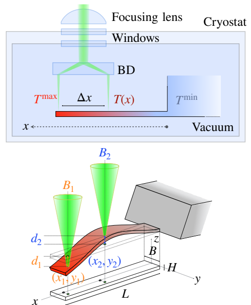
FIG. 1. Experiment setup: the flexion and torsion of a cantilever inside a cryostat are captured thanks to a differential interferometer [19–21]. A green laser beam ( \lambda = 532 \text{nm} ) is divided in two by a beam displacer BD and focused on the cantilever. The interferometer senses the vertical distance d_1 - d_2 between the beam B_1 close the cantilever tip and B_2 close to the center. The probing points are separated of \Delta x = x_1 - x_2 = 417 \mu\text{m} , \Delta y = 0 . The cantilever, in vacuum at 10^{-7} mbar, is monolithically clamped to its macroscopic chip which is thermalised at temperature T^{\text{min}} . When the laser power is low ( P < 1 \text{mW} ), we consider the system in thermal equilibrium. When the power is raised (10 to 40 \text{mW} ), a temperature gradient T(x) along the cantilever arises.
