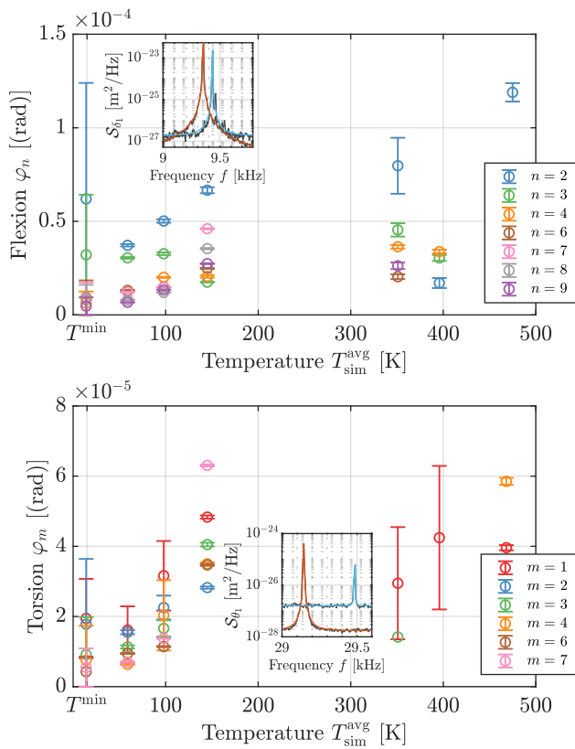
FIG. 4. Loss angles \varphi_n of flexural modes (a) and \varphi_m of torsional modes (b) with respect to the average temperature of the cantilever. Due to experimental constraints and low sample size, the fit of the experimental spectra are often hard to compute, thus we show only the results of fits with a \chi^2 < 3 . For most modes, the general trend is an increase of dissipation with increasing temperatures. In order to visually assess this, in the insets we show the peak of the PSD of the second modes in flexion and torsion, widening from low (cyan, T_{\text{sim}}^{\text{avg}} = 14 K) to high temperature (red, T_{\text{sim}}^{\text{avg}} = 474 K for flexion and T_{\text{sim}}^{\text{avg}} = 145 K for torsion).
