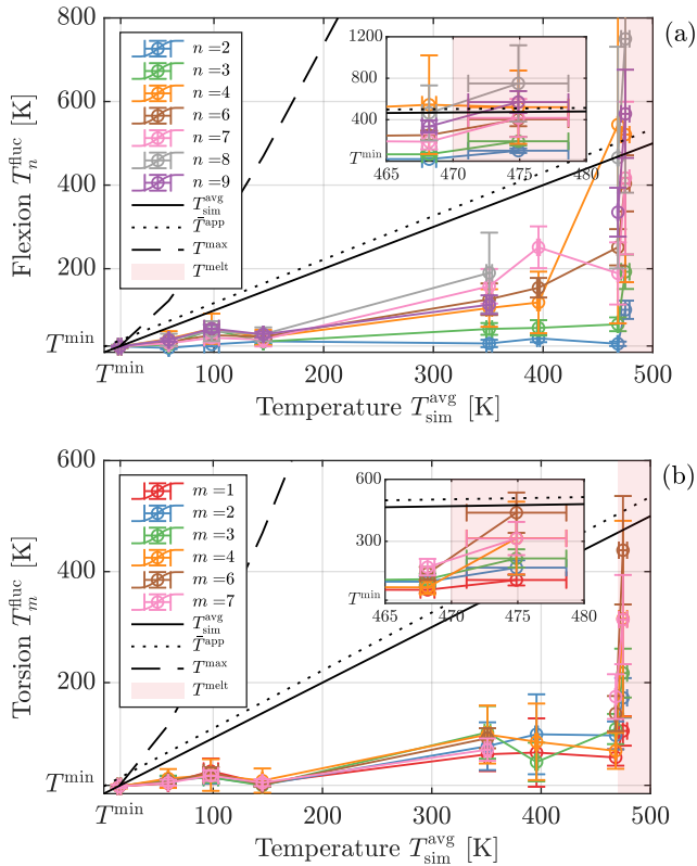
FIG. 3. Fluctuation temperature vs. average temperature, for flexion in (a) and torsion in (b). T_{\text{sim}}^{\text{avg}} (black solid line) and T^{\text{max}} (black dashed line) are evaluated from the measured frequency shift and the calibration function coming from the numerical simulation. The apparent temperature T^{\text{app}} (black dotted line) is evaluated from the measured frequency shift and the experimental calibration of the Young’s modulus temperature dependency. Albeit dependent of T^{\text{avg}} , the amplitude of fluctuations is well below those characteristics temperatures of the cantilever, showing a dearth of thermal noise. The red shaded area covers measurements where at least a partial melting of the cantilever occurred. It is remarkable that in this area T_{n,m}^{\text{fluc}} greatly increases for most modes of both families.
