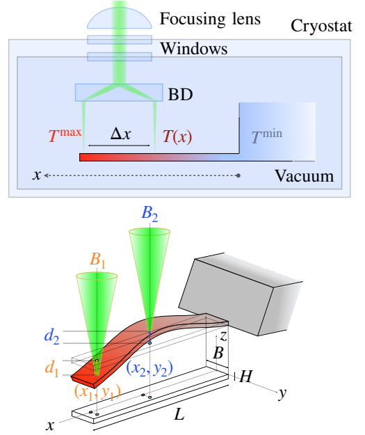
FIG. 1. Experiment setup: the flexion and torsion of a cantilever inside a cryostat are captured thanks to a differential interferometer [19–21]. A green laser beam ( \lambda = 532 \text{ nm} ) is divided in two by a beam displacer BD and focused on the cantilever. The interferometer senses the vertical distance d_1 - d_2 between the beam B_1 close the cantilever tip and B_2 close to the center. The probing points are separated of \Delta x = x_1 - x_2 = 417 \mu\text{m} , \Delta y = 0 . The cantilever, in vacuum at 10^{-7} mbar, is monolithically clamped to its macroscopic chip which is thermalised at temperature T^{\min} . When the laser power is low ( P < 1 \text{ mW} ), we consider the system in thermal equilibrium. When the power is raised (10 to 40 \text{ mW} ), a temperature gradient T(x) along the cantilever arises.
