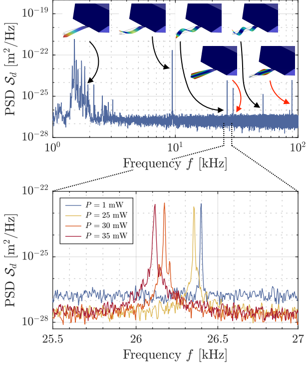
FIG. 2. Experimental thermal noise spectra. (a) The Power Spectrum Density (PSD) of d displays various resonance peaks, which we can distinguish between the flexural ones (black arrows) and torsional ones (red arrows). The first resonance n = 1 is plagued by low-frequency noise and is thus discarded in the analysis. (b) Increasing the laser power causes a redshift in the resonance frequencies of the modes (in this case n = 3 ) as the Young's modulus of silicon decreases with temperature.
