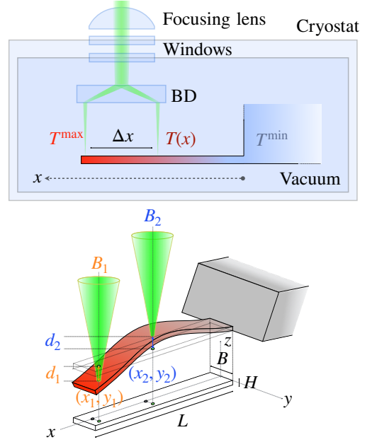
FIG. 1. (Color online) Experiment setup: the flexion and torsion of a cantilever inside a cryostat are captured thanks to a differential interferometer [19–21]. A green laser beam ( \lambda = 532 \text{ nm} ) is divided in two by a beam displacer BD and focused on the cantilever. The interferometer senses the vertical distance d_1 - d_2 between the beam B_1 close the cantilever tip and B_2 close to the center. The probing points are separated of \Delta x = x_1 - x_2 = 417 \mu\text{m} , \Delta y = 0 . The cantilever, in vacuum at 10^{-7} mbar, is monolithically clamped to its macroscopic chip which is thermalised at temperature T^{\min} . When the laser power is low ( P < 1 \text{ mW} ), we consider the system in thermal equilibrium. When the power is raised (10 to 40 \text{ mW} ), a temperature gradient T(x) along the cantilever arises.
