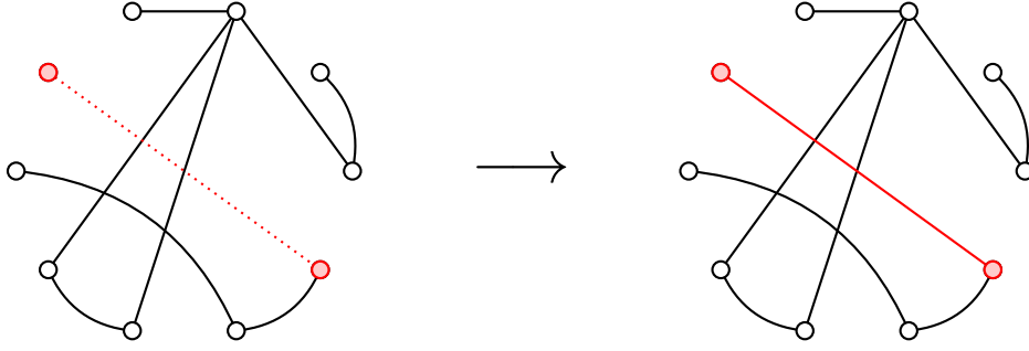
Figure 1 – One move of the dynamic of the dynamical inhomogeneous random graph. The red dotted edge which is absent on the left is the one chosen to be updated.
