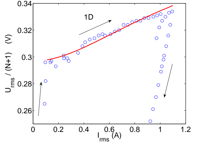
Fig. 5. Comparison between the AC characteristics measured at 1 MHz ( \circ ) in the chain of N = 9 beads, and the model ( - ) from Eq. (11) with A = 1.15 \mu\text{m}/\text{A} . Only the top part of the experimental curve is shown here to focus on the saturation regime.
