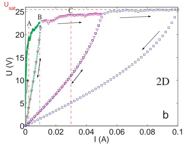
Fig. 3. (color online) Typical U - I characteristics. (a) 1D chain of N = 38 beads for an applied force F = 100 N. The dashed line U_{sat} \simeq 15.8 V corresponds to a saturation voltage per contact of V_o \equiv U_{sat}/(N+1) \simeq 0.4 V. The solid line is the theoretical down trajectory (see Ref. [8,14]). (b) 2D lattice of beads for an applied force F = 50 N. The dashed line corresponds to the saturation voltage U_{sat} \simeq 25.4 V. This value gives a measurement of the number of welded contact (see text). Different symbols correspond to different maximum applied current, I_{max} . The letters A, B and C correspond to the current maps of Figs. 4a, b and c.
