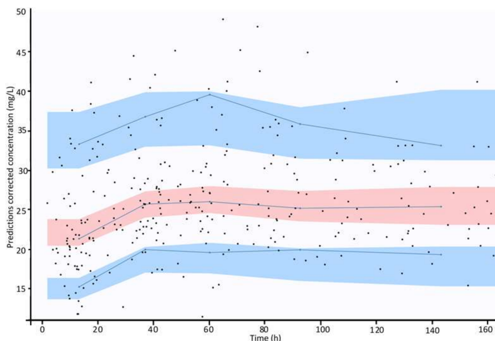
Figure 2. Internal validation of the model: prediction-corrected visual predictive checks.
