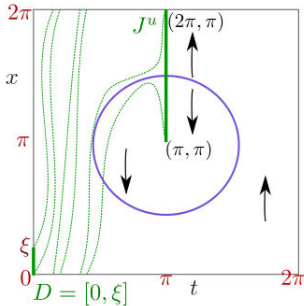
FIGURE 1.8 – The flow of the vector field (1.2) corresponding to the parameters (a, b, \mu) belonging to the zero boundary of the tongue, a = a_{0,k}(b) for a fixed \mu . The interval J^u corresponds to the half of the circle \{t = \pi\} and covers the repelling part of the slow curve. Its preimage D under the flow of Josephson equation is exponentially small in \mu . The slow curve is the violet curve.
