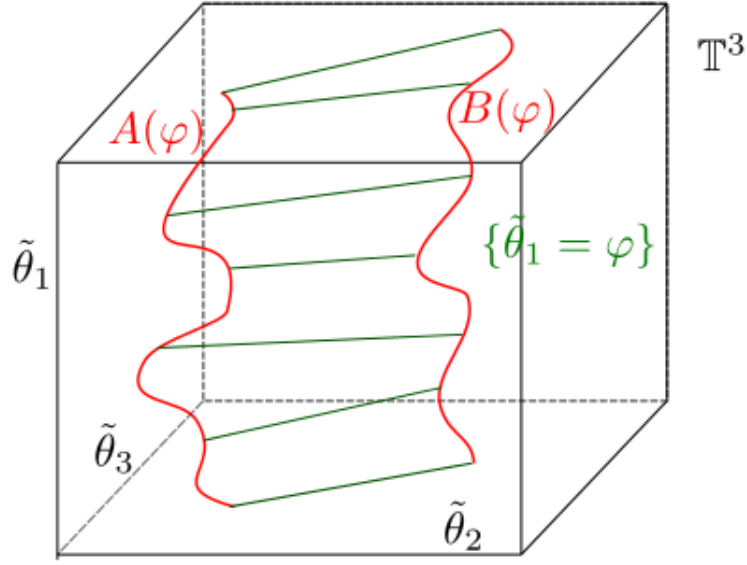
FIGURE 2.12 – The calculation of asymptotic velocity is related to the calculation of the flux of the vector field X through the cylinder foliated by intervals \theta_1 = \text{const} depicted on the picture. The cube on the picture is a fundamental domain of the torus \mathbb{T}^3 so its opposite sides are identified.
