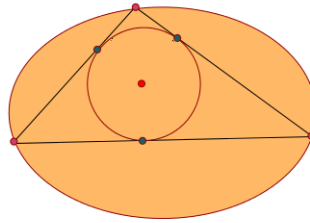
FIGURE 3.1 – The illustration for the main theorem : an ellipse, one of the periodic orbits, its incircle and the center of this circle. The locus of incenters is forming an ellipse.
