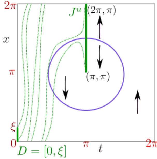
FIGURE 1.8 – The flow of the vector field (1.2) corresponding to the parameters (a, b, \mu) belonging to the zero boundary of the tongue, a = a_{0,k}(b) for a fixed \mu . The interval J^\mu corresponds to the half of the circle \{t = \pi\} and covers the repelling part of the slow curve. Its preimage D under the flow of Josephson equation is exponentially small in \mu . The slow curve is the violet curve.
