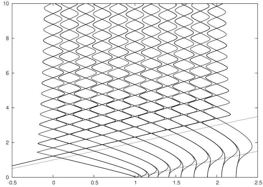
FIGURE 1.5 – The black lines correspond to the boundaries of Arnold tongues for Josephson equation on the parametric plane (a, b) corresponding to rotation numbers \rho = 0, 1, 2, \dots, 10 for \mu = 0.2
