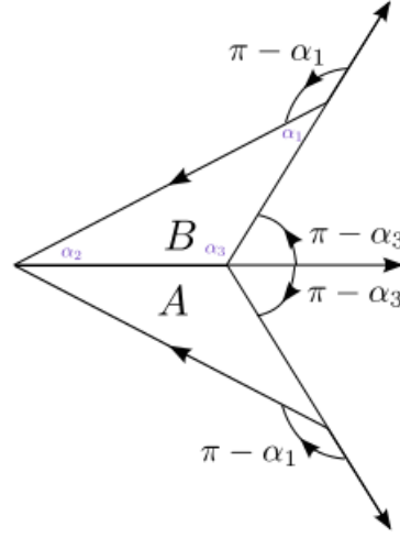
FIGURE 2.8 – Two positions corresponding to the singular points of the form \beta_{\text{sing}} on the hyperbolic plane : the positions in which the swiveling arm closes up into a triangle. This triangle has the sides of lengths |l_j|, j = 1, 2, 3 and the angles of values \alpha_j, j = 1, 2, 3 . The corresponding to singularities points on the torus \mathbb{T}^2 with coordinates (\tilde{\theta}_2, \tilde{\theta}_3) are the points A(-\pi + \alpha_3, -\pi + \alpha_1) and B(\pi - \alpha_3, \pi - \alpha_1) . Note that now the coordinates are defined as angles between the present direction of the interval and the positive direction of the previous interval in the chain. We suppose that the coordinate is growing when the angle changes counterclockwise.
