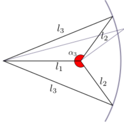
FIGURE 2.2 – For a fixed position of the first interval, the angles \theta_2 corresponding to the position of the second interval that correspond to the inequality |l_1 e^{i\theta_1} + l_2 e^{i\theta_2}| < |l_3| , are contained in the range (-\alpha_3, \alpha_3) where \alpha_3 is the angle in the triangle with the sides |l_j| . On the picture one can see two positions of the swiveling arm in which |l_1 e^{i\theta_1} + l_2 e^{i\theta_2}| = |l_3| .
