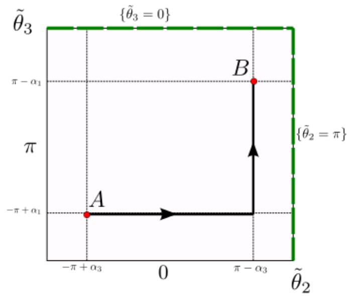
FIGURE 2.9 – A path of integration for a singular part of Lagrange form in the hyperbolic case on the two-torus with coordinates (\tilde{\theta}_2, \tilde{\theta}_3) . The path corresponds to turning first the second interval and then the third interval to come from one singular point to the other. Here the coordinates \tilde{\theta}_j, j = 2, 3 correspond to the relative positions of the intervals (with respect to a previous interval). The green paths \{\tilde{\theta}_3 = 0\} and \tilde{\theta}_2 = \pi are used after for the calculation of the periods of the regular part of Lagrangian 1-form.
