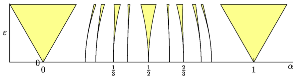
FIGURE 1.2 – Arnold tongues for a classical family (1.6) on the plane of parameters (a, \epsilon) : the tongues that are drawn on the picture are those corresponding to rational values with denominator no bigger than 5.
