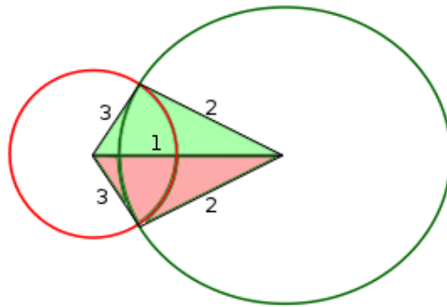
FIGURE 2.11 – The intersection of two convex discs gives two points that correspond to the vertices of two triangles with the sides of lengths l_1, l_2, l_3 .
