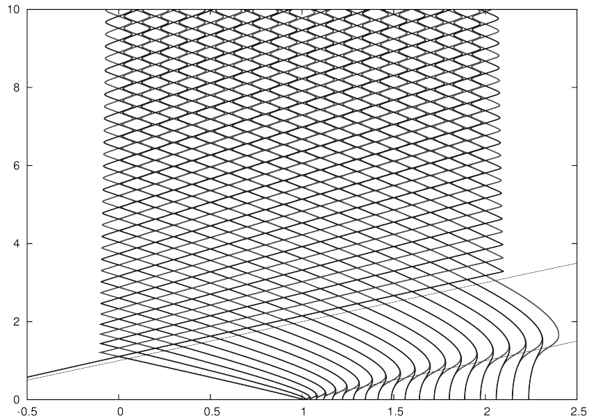
FIGURE 1.6 – By diminishing \mu and taking \mu = 0.1 one can see that the tongues become closer to each other, and the gaps between the tongues are impossible to detect with an eye
