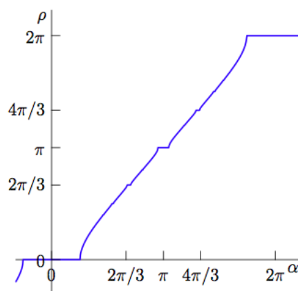
FIGURE 1.3 – A Cantor staircase for a standard Arnold family of circle diffeomorphisms (1.6) : the graph is a section of the picture on Figure 1.2 by a line \{\epsilon = \text{const}\}
