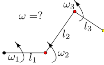
FIGURE 2.1 – A swiveling arm of type (l_1, l_2, l_3) rotating in a vector field (2.2) with N = 3 .
