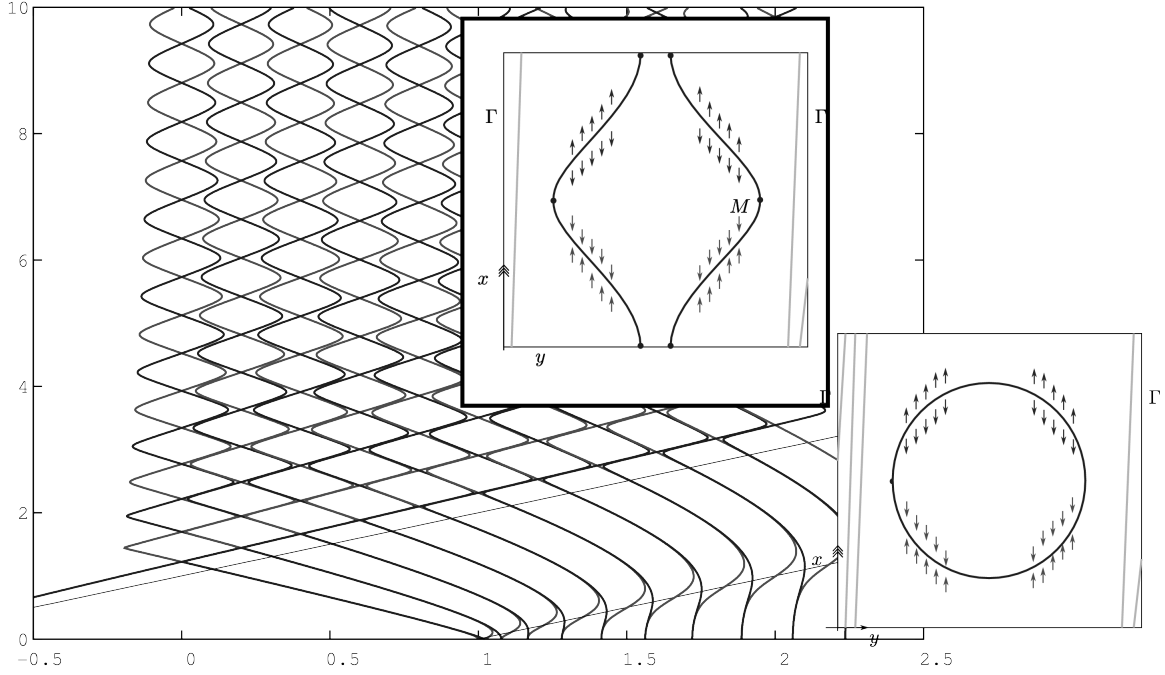
FIGURE 1.10 – The picture of domains A , B and C described euristically in Subsection 1.4.1. The domains B and C correspond to non-empty slow curves : the techniques of slow-fast systems are applied to study Arnold tongues, the domain A is much harder to study and almost nothing is known about the behaviour of the tongues in this domain.
