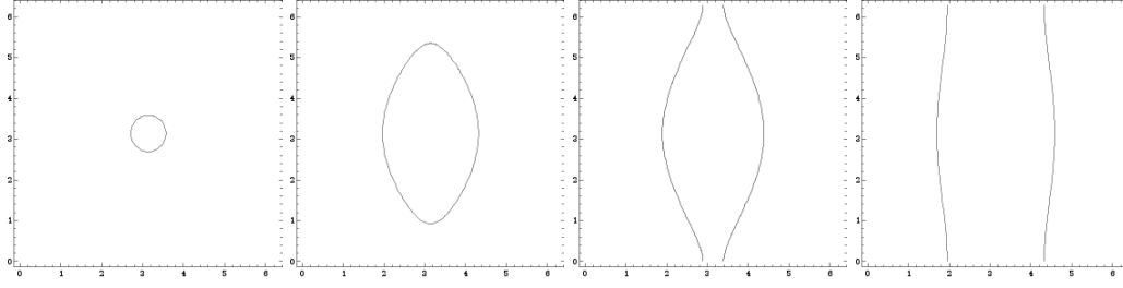
FIGURE 1.7 – A stop-motion movie showing the change of a slow curve with a fixed a and growing b . There is no slow curve for small b then it appears when b = a - 1 (it is a point in this case). The the slow curve continues growing and at b = a + 1 there is a new bifurcation : the curve starts intersecting itself. Then it falls into two non-intersecting homotopic circles that tend to torus meridians while b \rightarrow \infty
