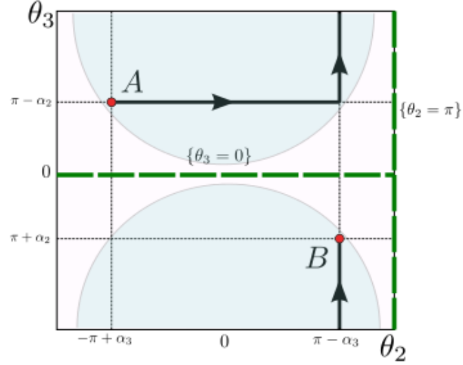
FIGURE 2.6 – A special path connecting the points A and B on the two-torus (chosen inside a blue disc used for a definition of the form \beta_{\text{sing}} ). The flux of the vector field X through this path is equal to the evaluation of the dipolar part of the form \beta on X . The paths corresponding to the generators in cohomology of the torus correspond to the periods of the regular part of the form \beta .
