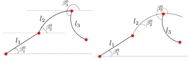
FIGURE 2.7 – Different ways to define the initial positions of the intervals : in the first case, with respect to the common horizontal direction (as an euclidian case where the translations exist) and with respect to the previous interval (in general case).
