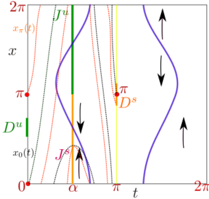
FIGURE 1.9 – The idea of the proof of Theorem 1.9 is shown on this Figure. The slow curve in the domain C (in violet) has two components – two circles. Under the supposition we make in the proof of Theorem 1.9 the picture is the following. The circle \{t = \alpha\} is divided into two parts : an attractive part J^s and a repelling part J^u . The trajectories of all the points of the transversal \{t = 0\} except for an exponentially small interval D^u will cross the section J^s : so the trajectories x_0(t) and x_\pi(t) will be very close once they have stayed some time near the attracting part of the slow curve. And since x_0(\pi) = \pi then, by a small change of parameters one can obtain x_\pi(\pi) = \pi and pass to the neighboring tongue.
