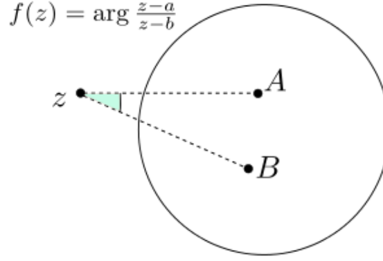
FIGURE 2.4 – Multivalued function f(z) = \arg \frac{z-A}{z-B} is well-defined outside the big ball containing points A and B as an angle between two rays connecting z to A and to B correspondingly (there is a continuous determination for this function)
