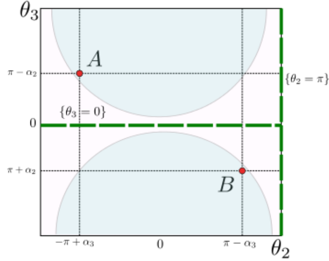
FIGURE 2.5 – The torus \mathbb{T}^2 corresponding to the position of the swiveling arm with three joints in the assumption \omega_1 = 0 . Points A, B \in \mathbb{T}^2 corresponding to singularities of the form \beta are put inside the (blue) disk and hence the form \beta_{\text{sing}} is defined as a dipolar form on the torus.
