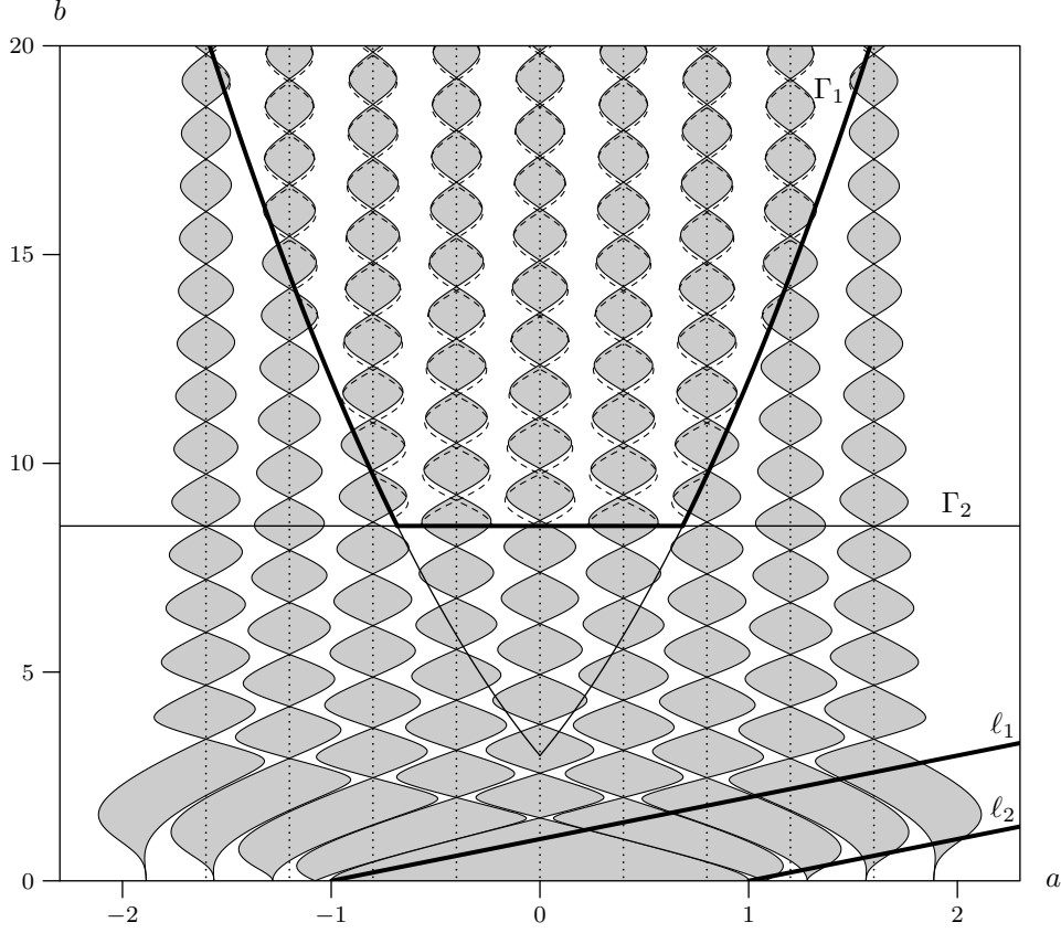
Figure 1: Arnold tongues of Josephson equation in the domain on the plane of parameters (a, b) for a fixed \mu = 0.4 .
