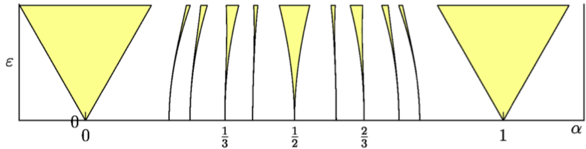
FIGURE 1.2 – Arnold tongues for a classical family (1.6) on the plane of parameters (a, \varepsilon) : the tongues that are drawn on the picture are those corresponding to rational values with denominator no bigger than 5.
