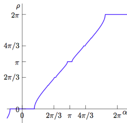
FIGURE 1.3 – A Cantor staircase for a standard Arnold family of circle diffeomorphisms (1.6): the graph is a section of the picture on Figure 1.2 by a line \{\varepsilon = \text{const}\}
