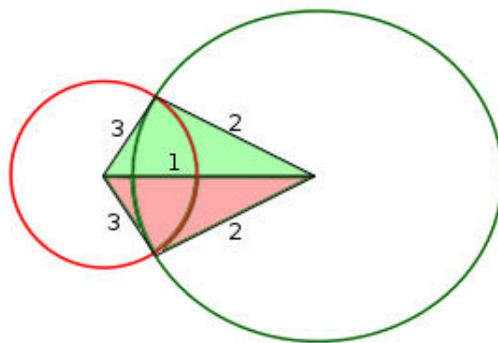
FIGURE 2.11 – The intersection of two convex discs gives two points that correspond to the vertices of two triangles with the sides of lengths l_1, l_2, l_3 .
