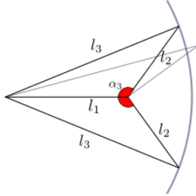
FIGURE 2.2 – For a fixed position of the first interval, the angles \theta_2 corresponding to the position of the second interval that correspond to the inequality |l_1e^{i\theta_1} + l_2e^{i\theta_2}| < |l_3| , are contained in the range (-\alpha_3, \alpha_3) where \alpha_3 is the angle in the triangle with the sides |l_j| . On the picture one can see two positions of the swiveling arm in which |l_1e^{i\theta_1} + l_2e^{i\theta_2}| = |l_3| .
